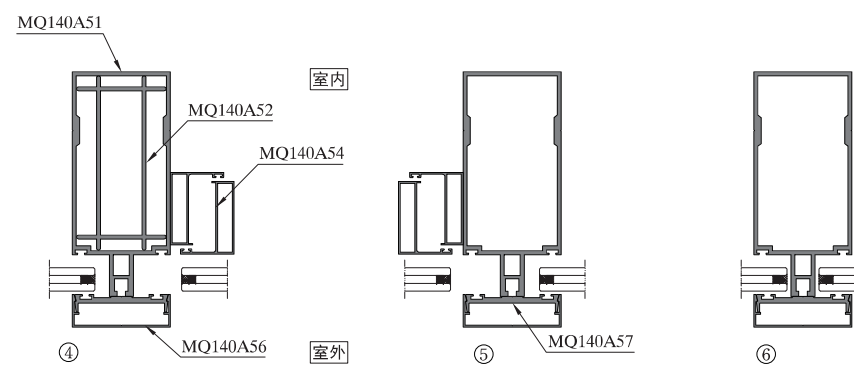
图中所示型材截面、装配、编号、尺寸及重量仅供参考。如有疑问，请向本公司查询。 Information above just for your reference. Please contact us if you have any questions, Thank you!
