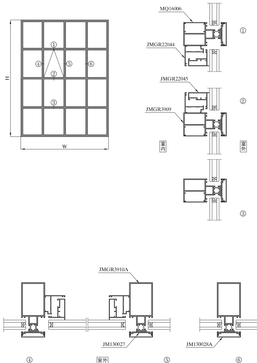
图中所示型材截面、装配、编号、尺寸及重量仅供参考。如有疑问，请向本公司查询。 Information above just for your reference. Please contact us if you have any questions, Thank you!
