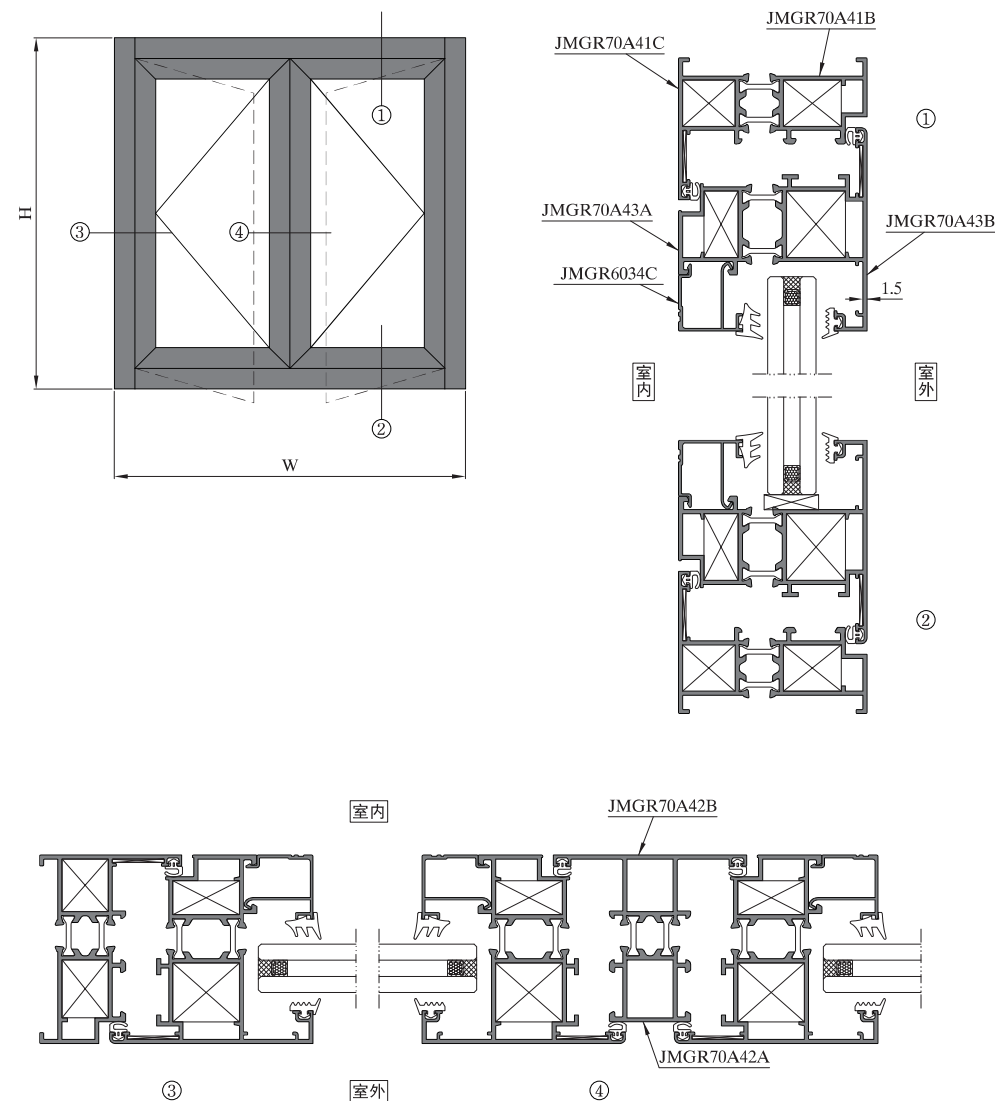
图中所示型材截面、装配、编号、尺寸及重量仅供参考。如有疑问，请向本公司查询。 Information above just for your reference. Please contact us if you have any questions, Thank you!
